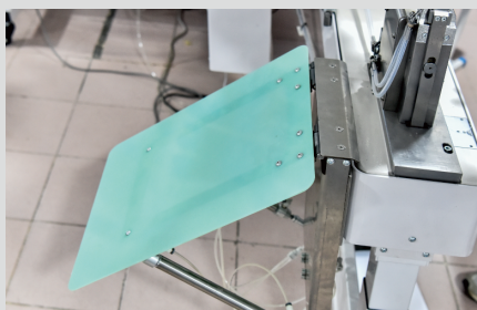
可选配气动辅助架，轻松应对大件材料的缝纫。 Optional pneumatic auxiliary frame, easy to handle sewing of large materials.
